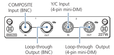
LMD-2450W/LMD-2050W Option Slots
