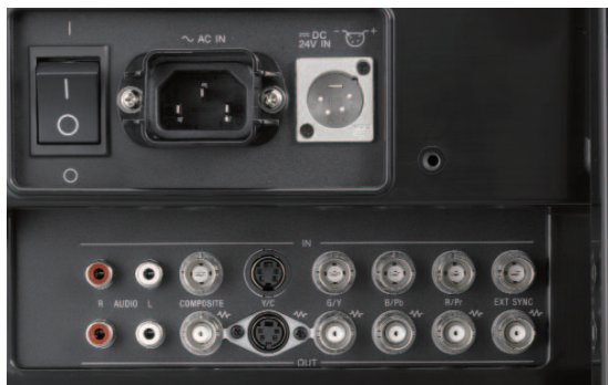
LMD-2450W/LMD-2050W Connector Panel
