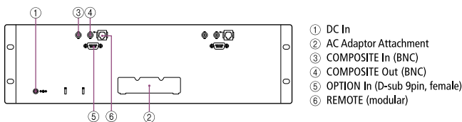
LMD-5320 Connector Panel
