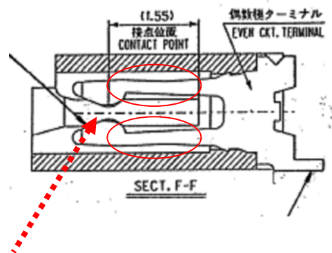
Cross-section drawing of Connector for Non RoHS compliant models (A' rank)
