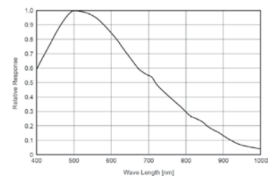
Spectral Sensitivity for FO124TB
